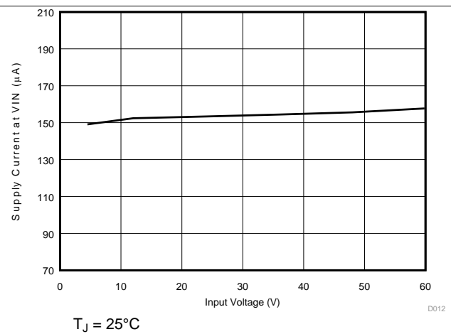
Figure 18. I_{(VIN)} Supply Current vs Input Voltage
