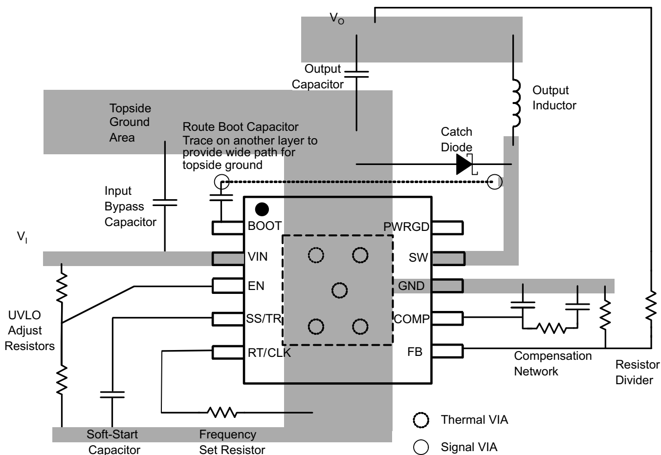
Figure 68. PCB Layout Example
