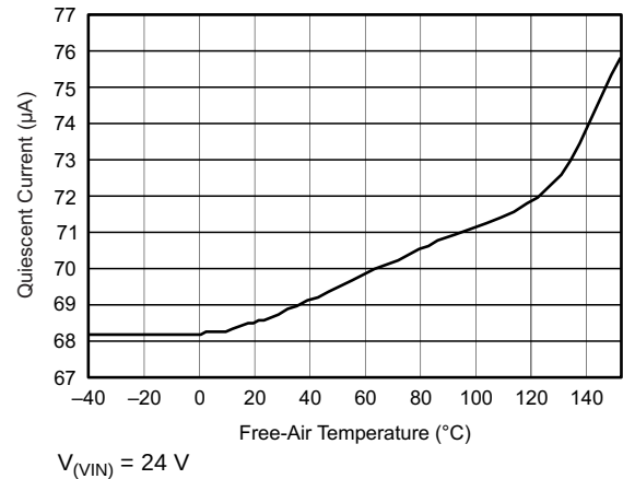
Figure 7. LPM, Quiescent Current Variation with Temperature
