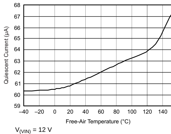
Figure 6. LPM, Quiescent Current Variation With Temperature
