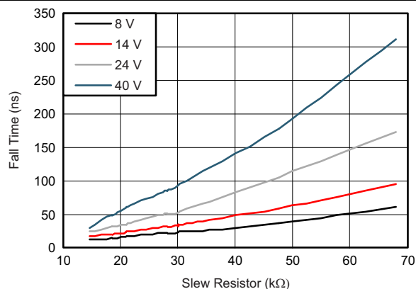
Figure 17. FET Fall Time
