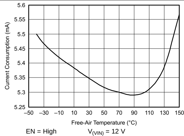
Figure 10. Current Consumption vs Temperature
