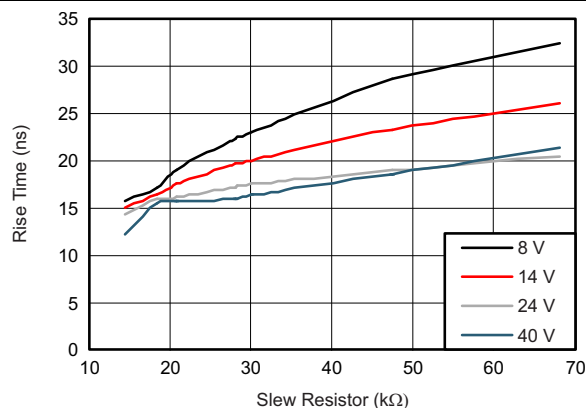
Figure 16. FET Rise Time
