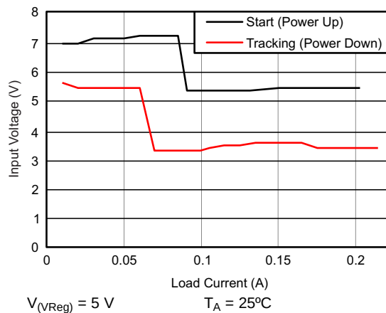
Figure 5. Output-Voltage Tracking
