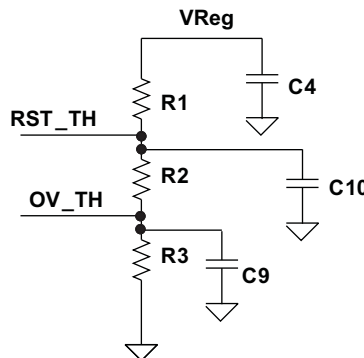
Figure 18. Resistor Network and Noise Filters
