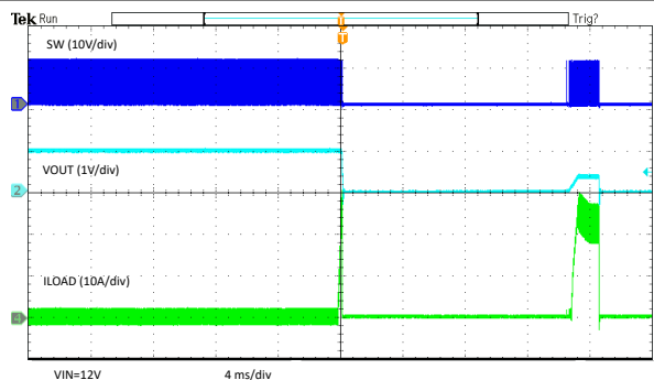
Figure 7-22. Overcurrent Protection – Hiccup and Recover
