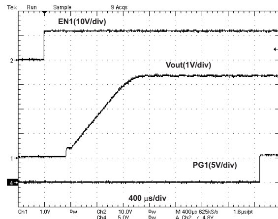
Figure 10. VO1=3.3V, PG1
