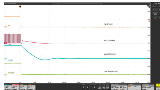
Figure 9-13. Shutdown With EN
