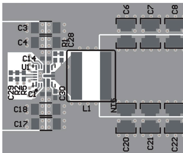
Figure 9-14. Layout Recommendation
