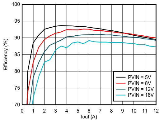
Figure 9-2. Efficiency - FCCM
