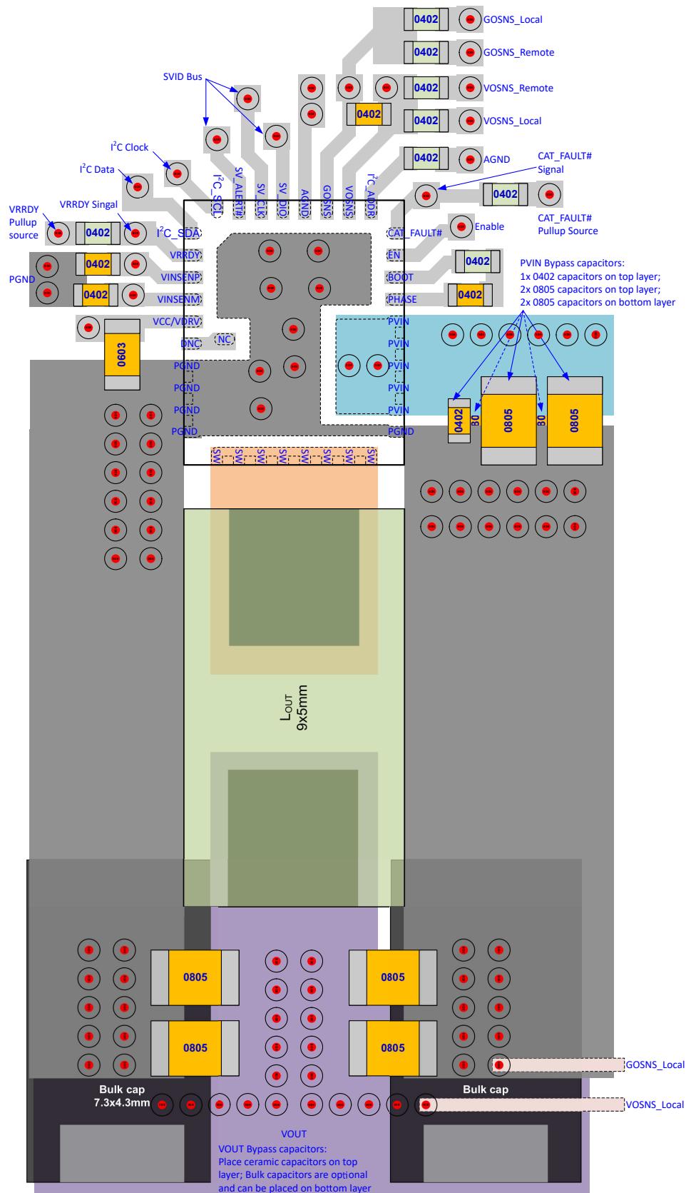
Figure 8-20. Layout Recommendation
