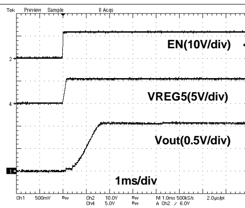
Figure 14. Start-Up Waveform
