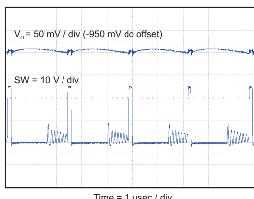
Figure 16. DCM Voltage Ripple at Output
