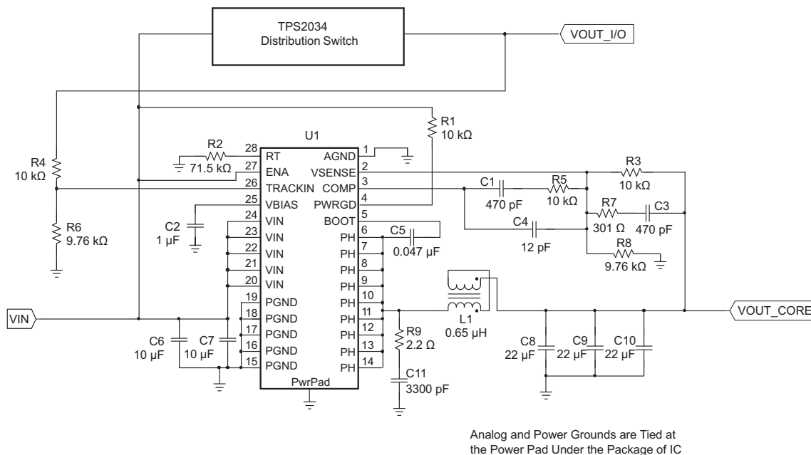
Figure 21. 3.3-V Small Size, High Frequency Design
