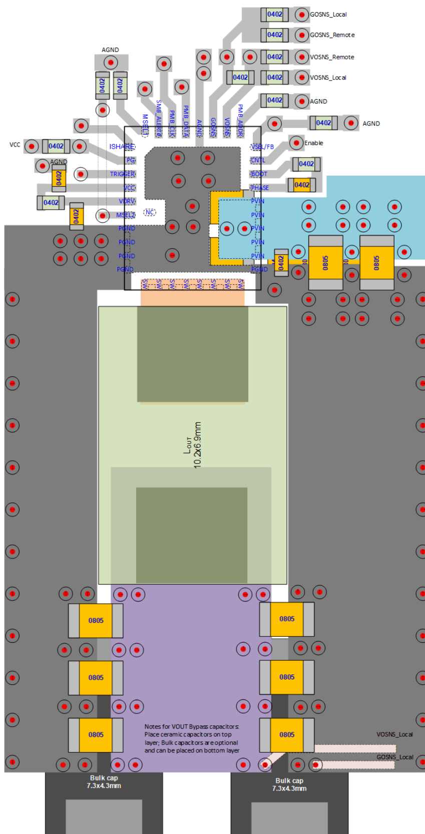
Figure 8-8. Layout Recommendation
