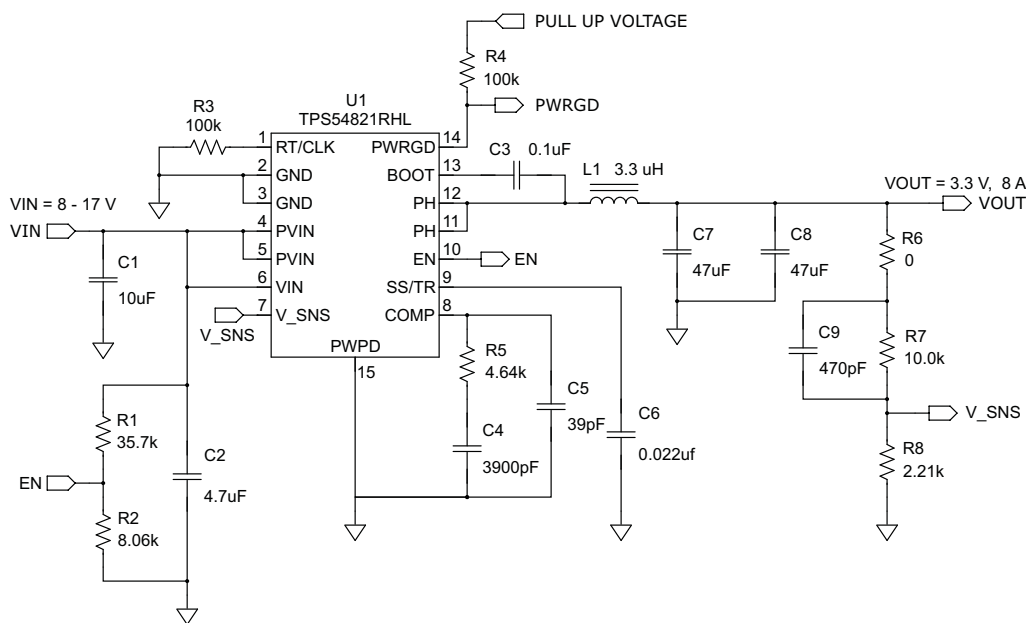
Figure 29. Typical Application Circuit
