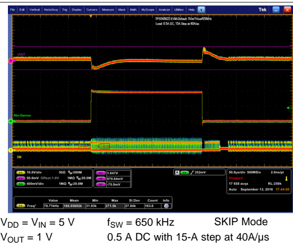
Figure 23. Transient Response Peak-to-Peak
