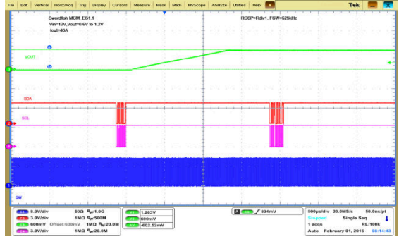
Figure 8-5. VOUT Command
