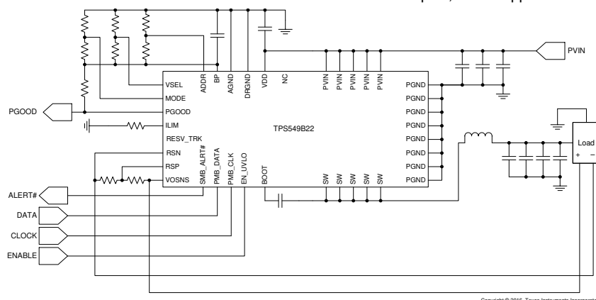
Simplified Application
