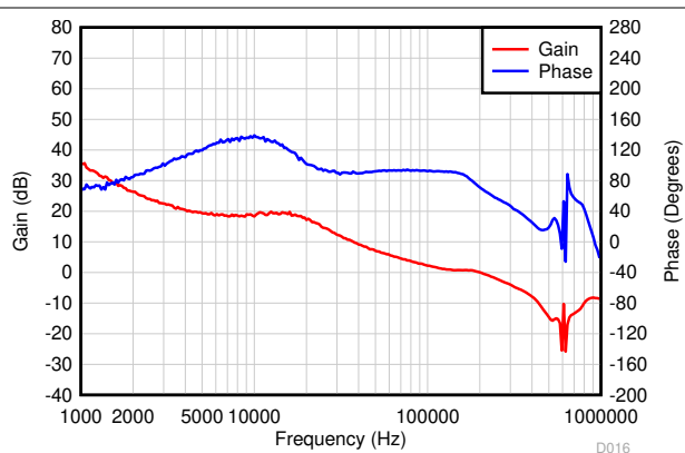
Figure 6-20. Frequency Response, 20 A Load
