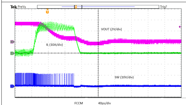
Figure 6-21. Overcurrent Protection
