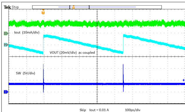
Figure 6-19. Vout Ripple, Skip-mode, 10mA Load
