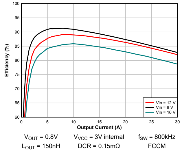
Figure 7-3. Efficiency – FCCM
