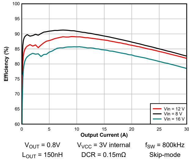
Figure 7-2. Efficiency – Skip-mode
