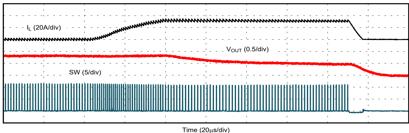
Figure 6-5. Overcurrent Protection
