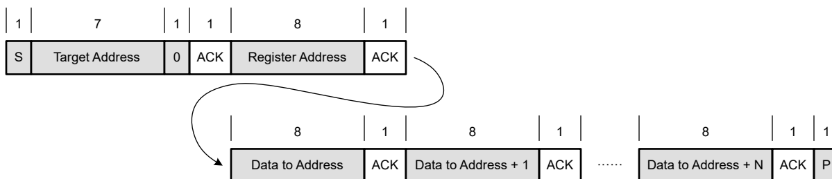
Figure 6-13. Multibyte Write
