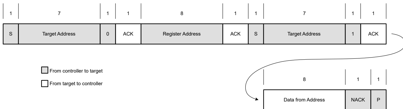
Figure 6-12. Single-Byte Read
