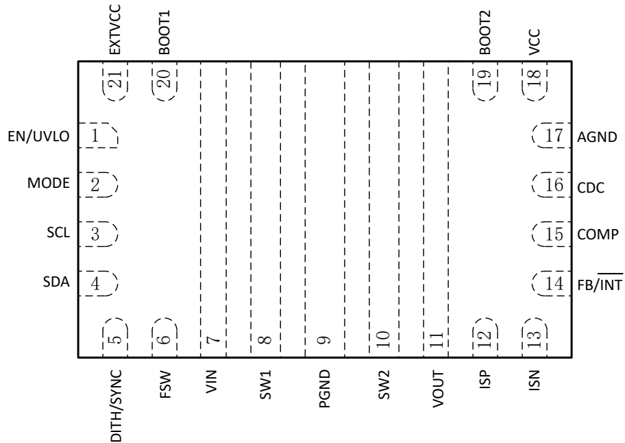
Figure 4-1. 21-Pin VQFN-HR RYQ Package (Transparent Top View)
