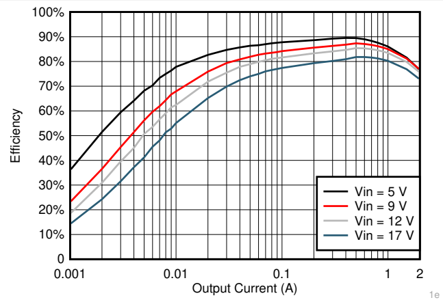
Figure 7-10. V_{OUT} = 1.05\text{-V} Efficiency, L = 2.2\text{ }\mu\text{H}
