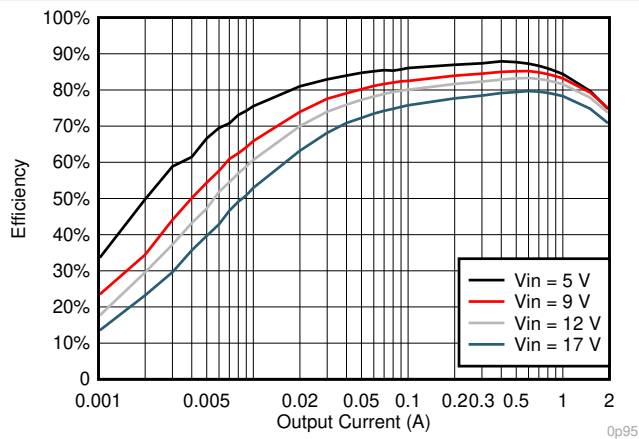
Figure 7-9. V_{OUT} = 0.95\text{-V} Efficiency, L = 2.2\text{ }\mu\text{H}
