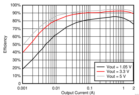
TPS562202S Efficiency
