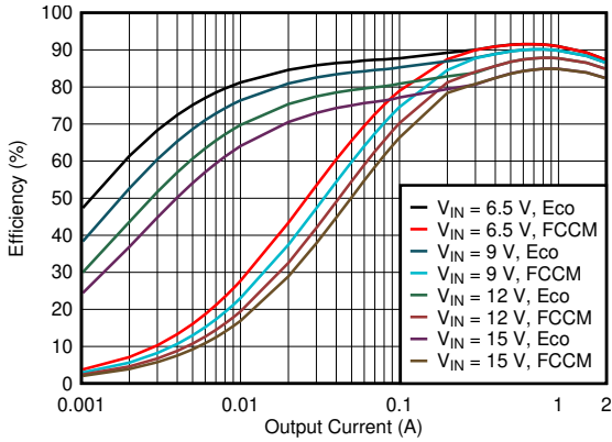
Figure 6-13. V_{OUT} = 1.05\text{-V} Efficiency, L = 2.2\text{ }\mu\text{H}
