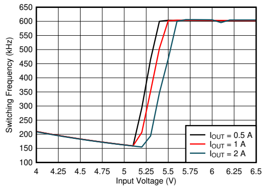
Figure 7-4. Frequency Foldback at Dropout ( V_{OUT} = 5 V)
