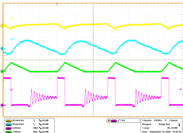
Figure 8-8. Steady State Waveforms, I_{OUT} = 0.2 A
