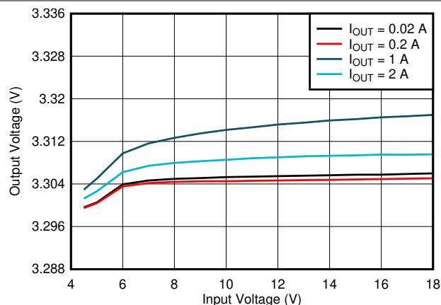
Figure 8-4. Line Regulation
