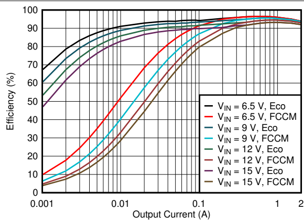
Figure 8-2. Efficiency
