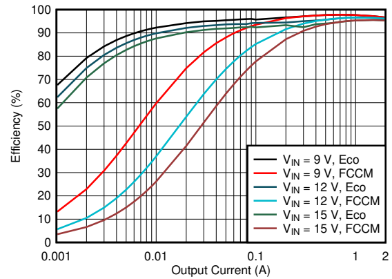
Figure 6-16. V_{OUT} = 7\text{-V} Efficiency, L = 5.6\text{ }\mu\text{H}
