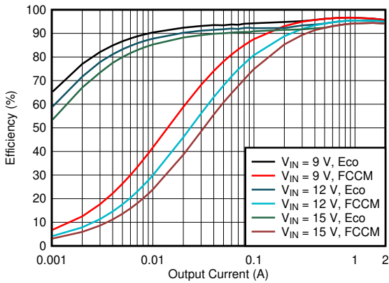
Figure 6-15. V_{OUT} = 5\text{-V} Efficiency, L = 5.6\text{ }\mu\text{H}
