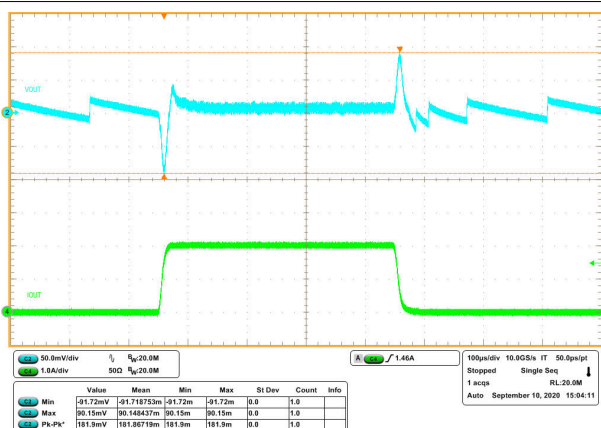
Figure 8-11. Transient Response 0 to 2 A with Slew Rate of 0.25 A/μs (Eco-mode)
