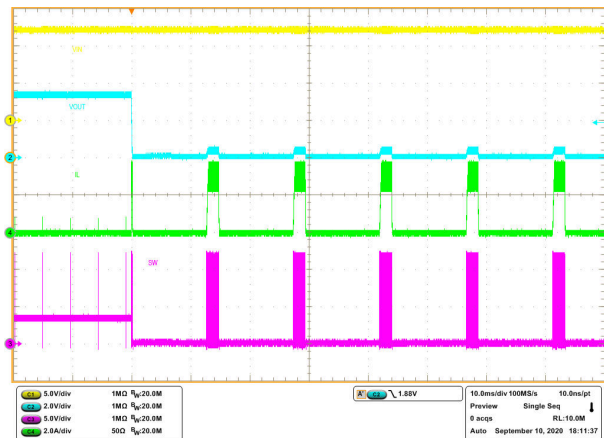
Figure 8-20. Output Short Protection
