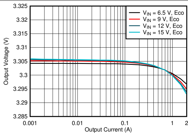
Figure 8-3. Load Regulation
