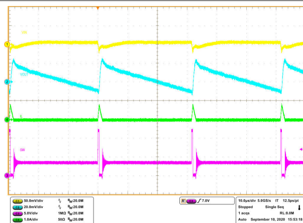
Figure 8-7. Steady State Waveforms, I_{OUT} = 0.02\text{ A}
