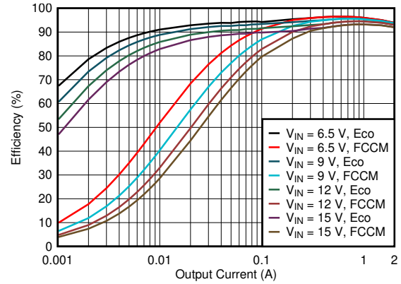
Figure 6-14. V_{OUT} = 3.3\text{-V} Efficiency, L = 4.7\text{ }\mu\text{H}
