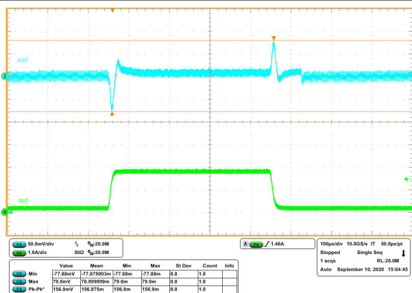
Figure 8-13. Transient Response 0.2 to 1.8 A with Slew Rate of 0.25 A/μs (Eco-Mode)
