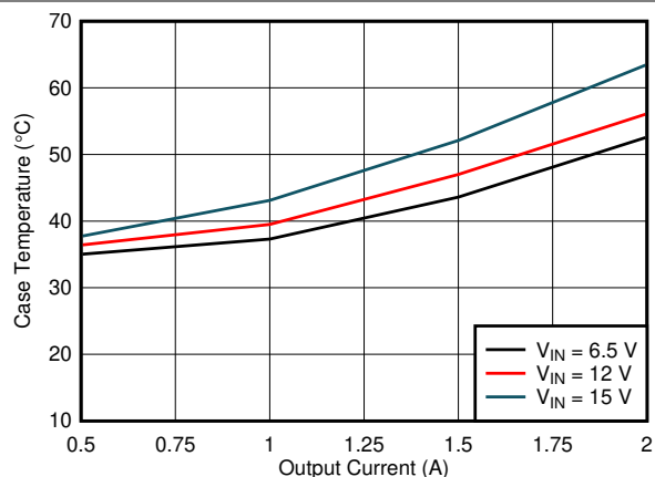
Figure 8-5. Case Temperature Rise vs Load Current
