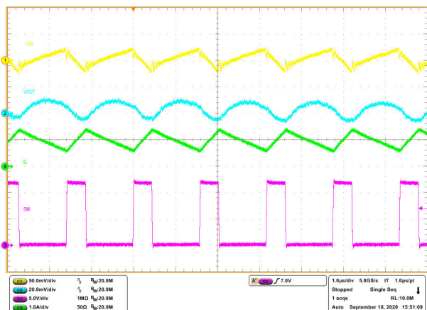
Figure 8-9. Steady State Waveforms, I_{OUT} = 1 A
