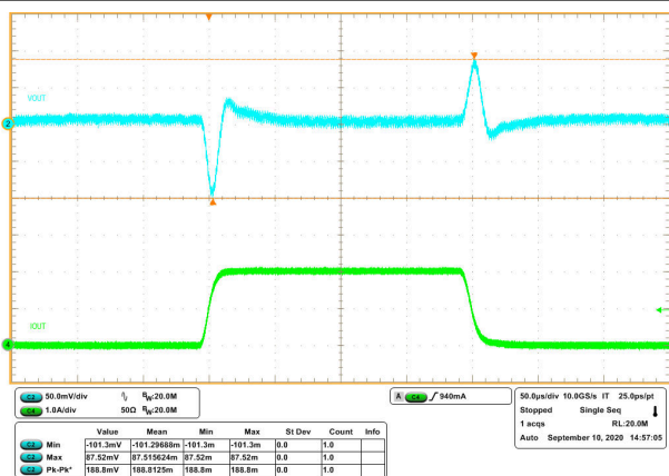
Figure 8-12. Transient Response 0 to 2 A with Slew Rate of 0.25 A/μs (FCCM)
