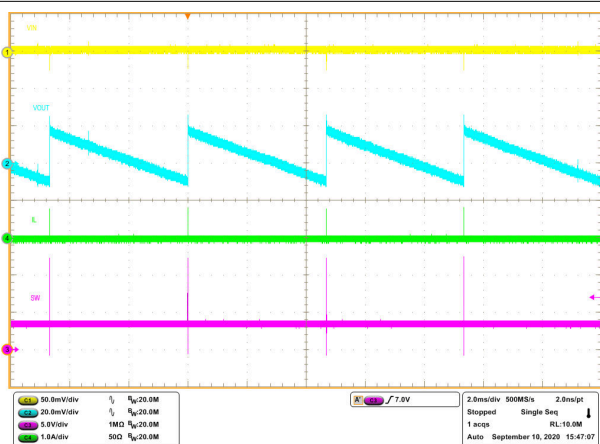
Figure 8-6. Steady State Waveforms, I_{OUT} = 0\text{ A}
