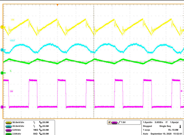
Figure 8-10. Steady State Waveforms, I_{OUT} = 2 A
