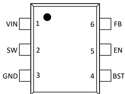
Figure 5-1. 6-Pin SOT563 DRL Package (Top View)
