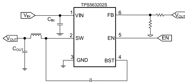
Simplified Schematic
