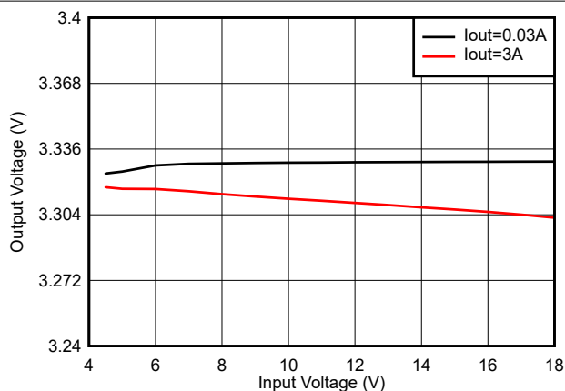
Figure 8-4. Line Regulation
