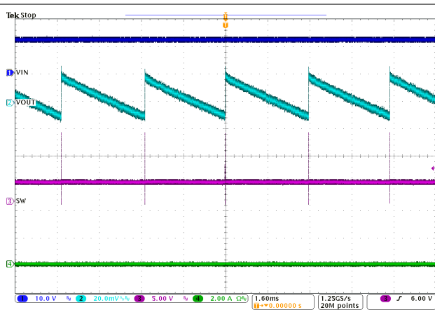
Figure 8-6. Steady State Waveforms, I_{OUT} = 0\text{ A}
