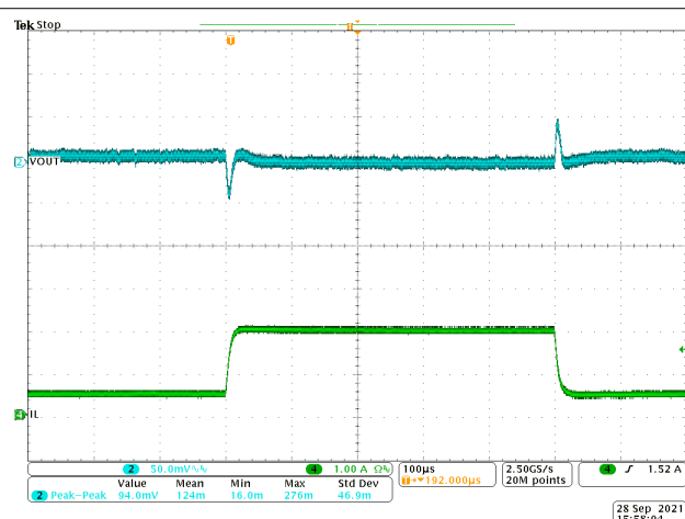
Figure 8-11. Transient Response 0.5 to 2 A with Slew Rate of 2.5 A/µs
