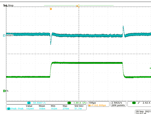
Figure 8-13. Transient Response 1.5 to 3 A with Slew Rate of 2.5 A/µs
