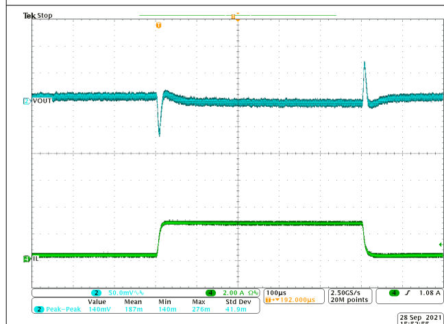
Figure 8-10. Transient Response 0.3 to 2.7 A with Slew Rate of 2.5 A/µs
