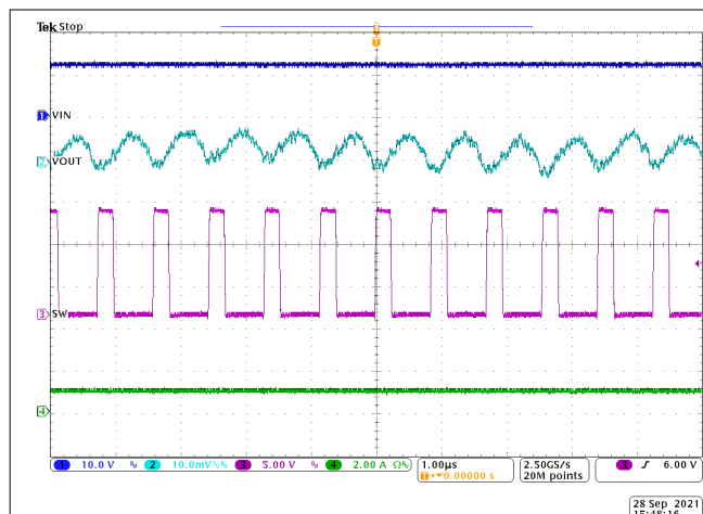
Figure 8-8. Steady State Waveforms, I_{OUT} = 1.0 A
