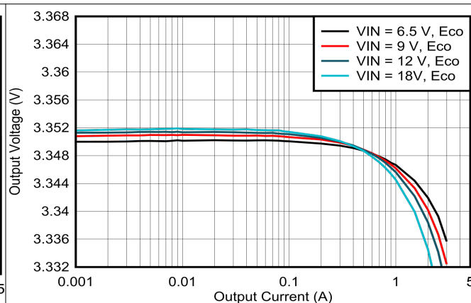
Figure 8-3. Load Regulation
