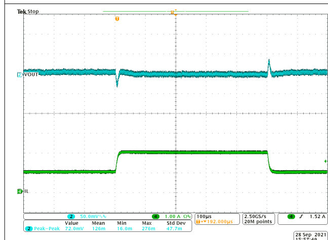
Figure 8-12. Transient Response 1 to 2 A with Slew Rate of 2.5 A/µs
