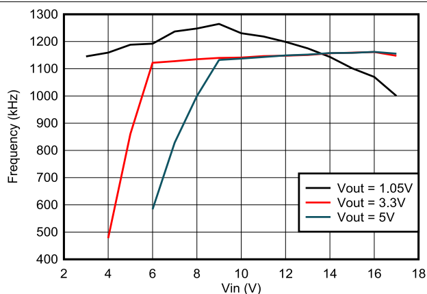
Figure 6-8. Frequency vs Input Voltage, I_{OUT} = 3\text{ A}
