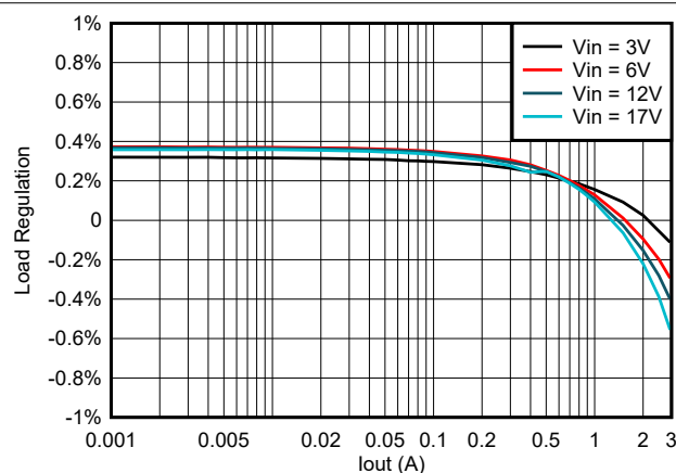
Figure 8-5. TPS563257 Load Regulation vs Loading
