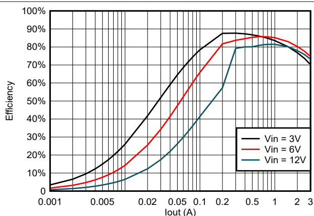
Figure 6-12. TPS563257 Efficiency at 0.6\text{ V}_{OUT} with a 0.68\text{-}\mu\text{H} Inductor
