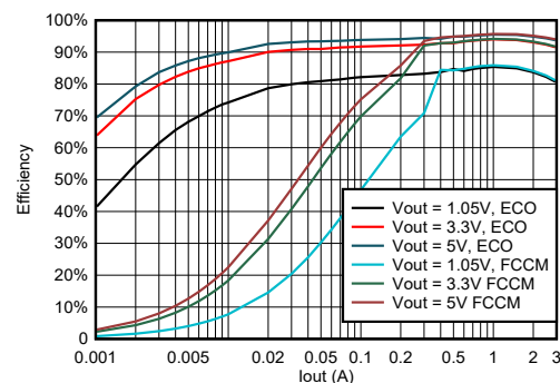
TPS56325x Efficiency at V_{IN} = 12\text{ V}
