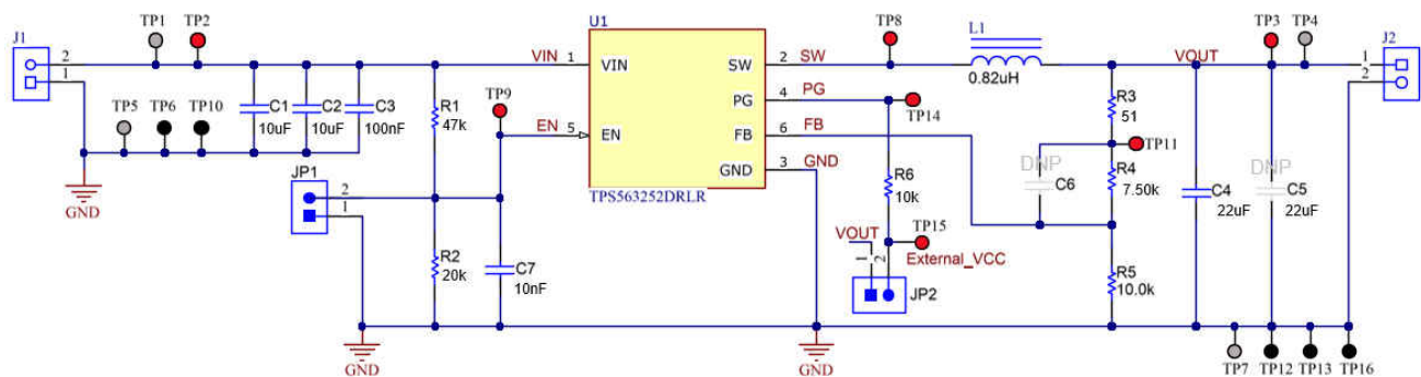
Figure 8-1. Schematic
