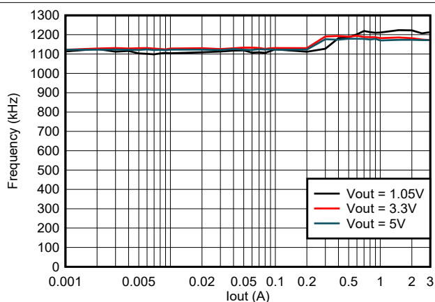
Figure 6-10. TPS563257 Frequency vs Loading, V_{IN} = 12\text{ V}
