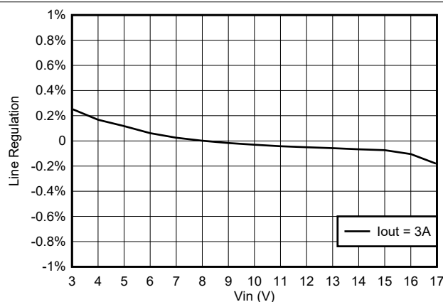
Figure 8-7. TPS563257 Line Regulation vs V_{IN}
