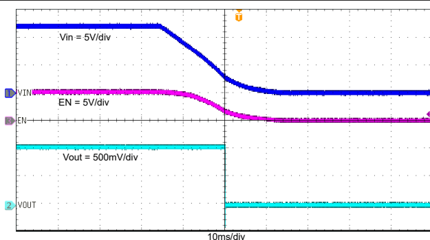
Figure 8-18. Shutdown with V_{IN} Falling, I_{OUT} = 3\text{ A}
