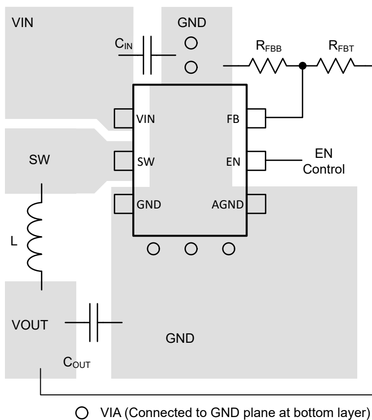
Figure 10-1. Suggested Layout
