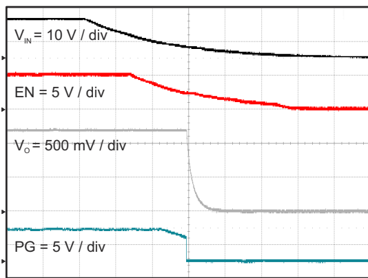
Figure 8-16. Shut Down Relative to V_{IN} Falling
