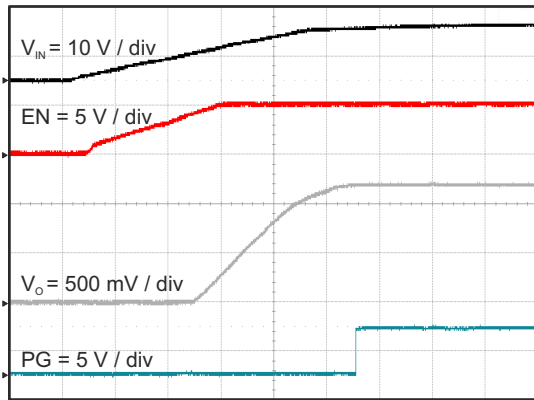
Figure 8-14. Start Up Relative to V_{IN} Rising
