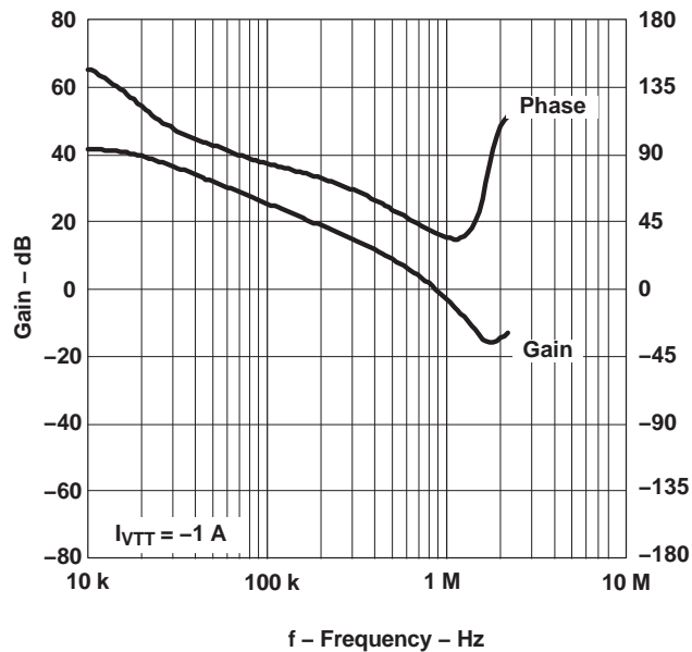
VTT BODE PLOT, SOURCE (DDR2) GAIN AND PHASE vs FREQUENCY
