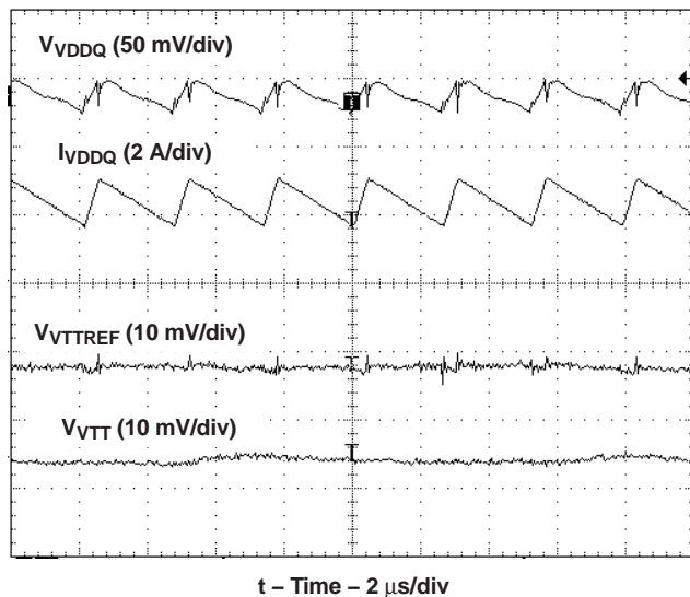
Figure 26. Ripple Waveforms - Heavy Load Condition
