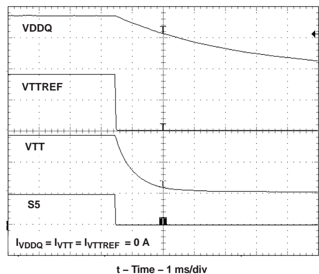
Figure 32. Soft-Stop Waveforms Non-Tracking Discharge
