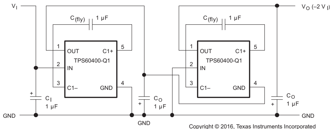
Figure 30. Doubling Inverter
