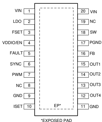
Figure 5-1. PWP Package 20-Pin HTSSOP With Exposed Thermal Pad Top View
