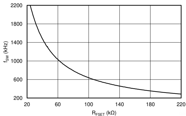
Figure 6-6. Boost Switching Frequency f_{SW} vs R_{ISET}
