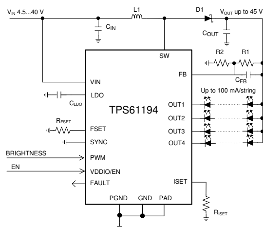
Simplified Schematic
