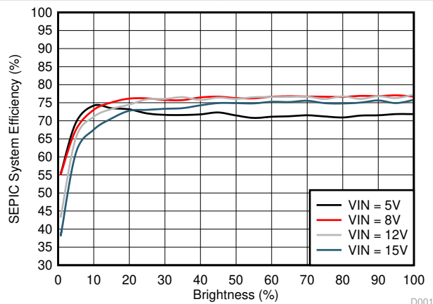
Figure 8-7. SEPIC Efficiency
