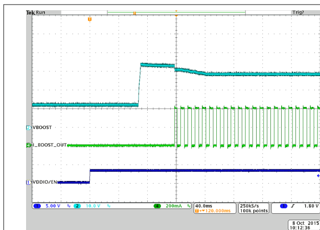
Figure 8-4. Typical Start-Up
