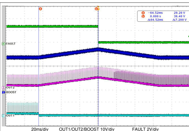
Figure 8-5. Open LED Fault
