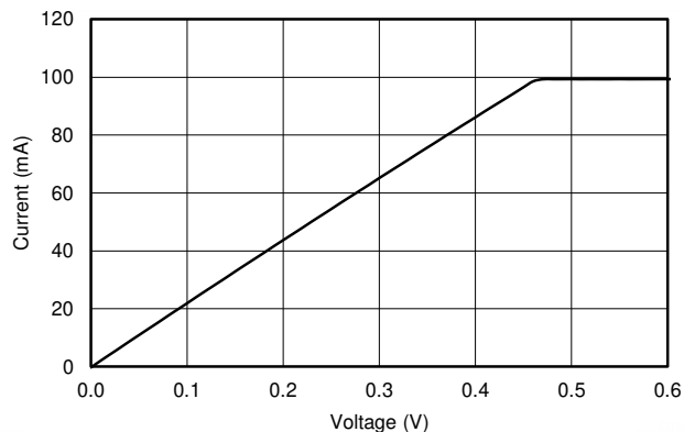
Figure 6-8. LED Current Sink Saturation Voltage
