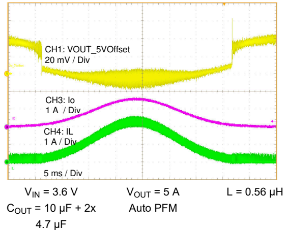
Figure 9-5. Load Sweep
