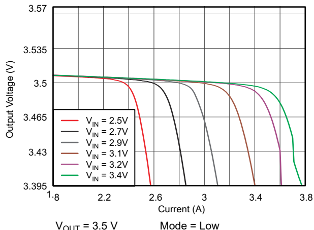
Figure 10-29. TPS61282D DC Output Voltage vs Output Current
