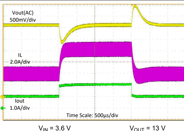
Figure 9-7. Load Transient ( I_{OUT} = 1\text{ to }2\text{ A} )
