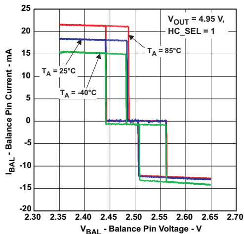
Figure 23. Balancing Current vs Balance Pin Voltage
