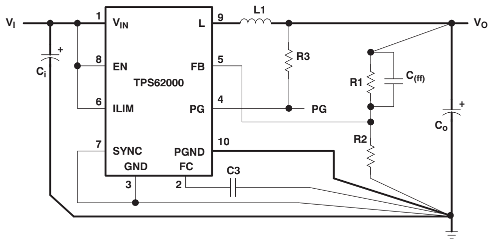
Figure 19. Layout Diagram
