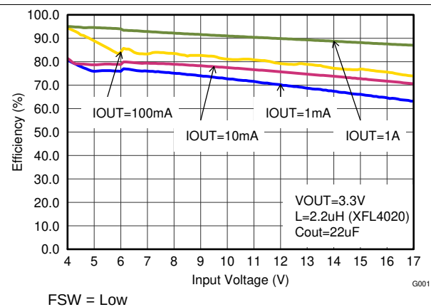
Figure 16. Efficiency versus Input Voltage
