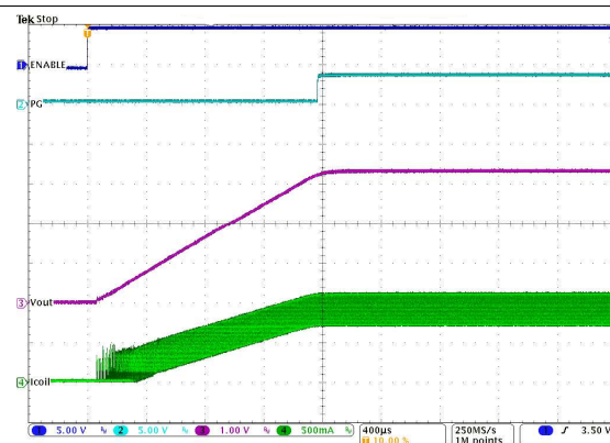
Figure 39. Start-up Into 1 A
