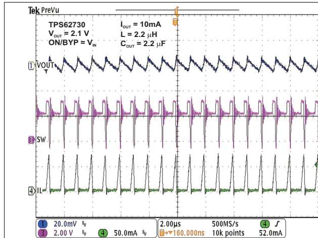
Figure 19. DC-DC Mode Operation I_{OUT} = 10 mA
