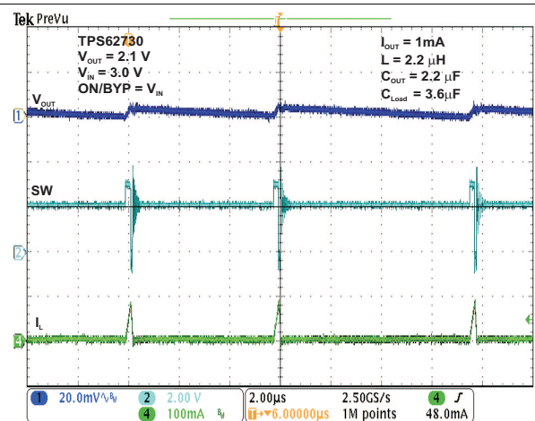
Figure 20. DC-DC Mode Operation I_{OUT} = 1 mA
