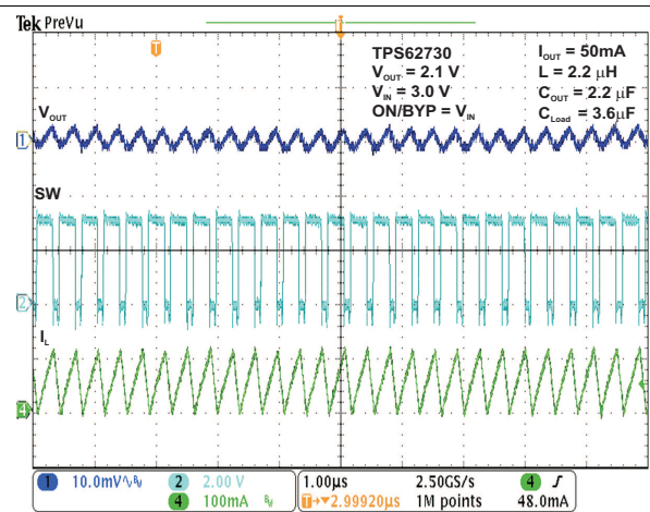
Figure 22. DC-DC Mode Operation I_{OUT} = 50 mA
