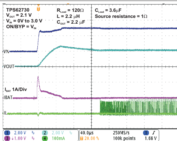
Figure 27. Start-Up Behavior
