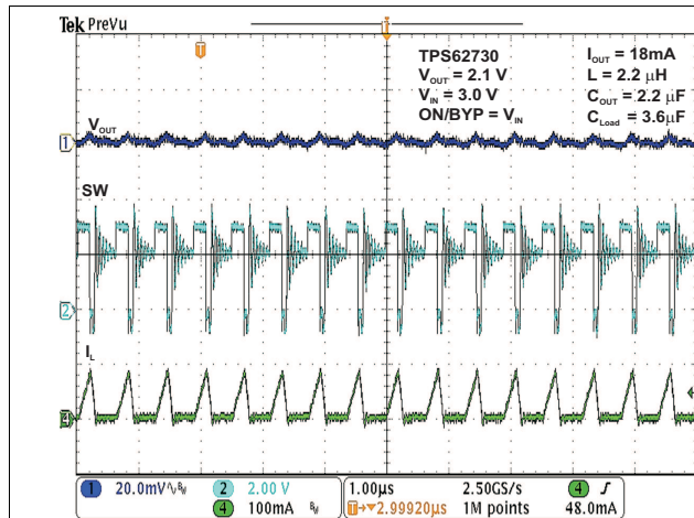
Figure 21. DC-DC Mode Operation I_{OUT} = 18 mA
