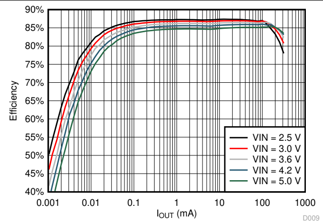
Figure 9-5. Efficiency vs Load Current; V_{OUT} = 1.8\text{ V}
