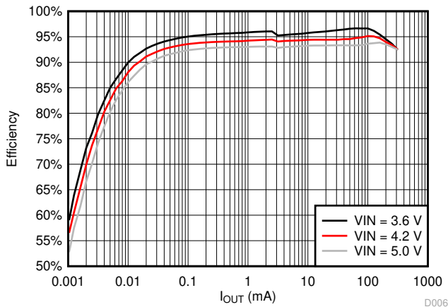
Figure 9-2. Efficiency vs Load Current, V_{OUT} = 3.3\text{ V}
