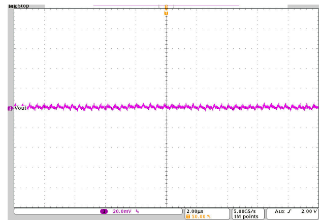
Figure 10-45. Output Voltage Ripple
