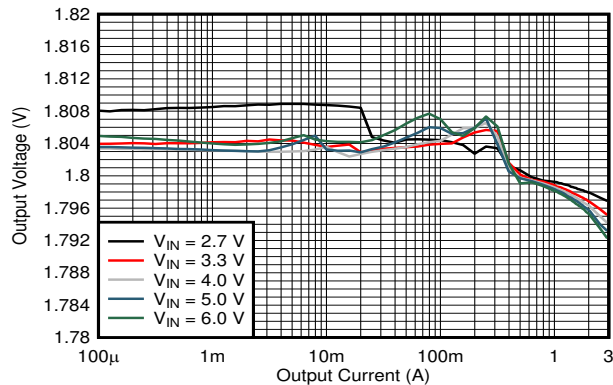
Figure 9-10. Output Voltage Versus Output Current
