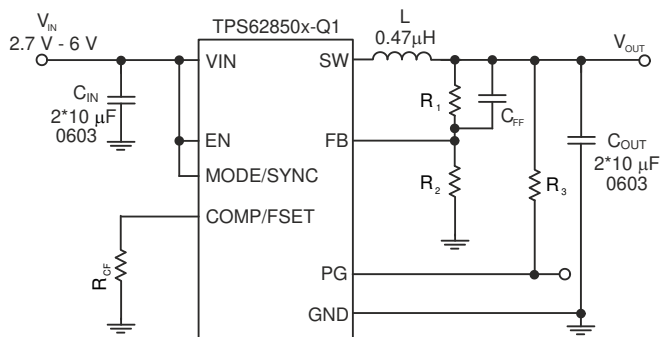
Simplified Schematic
