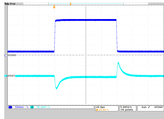
Figure 9-29. Load Transient Response
