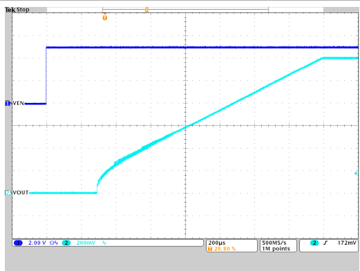
Figure 9-52. Start-Up Timing
