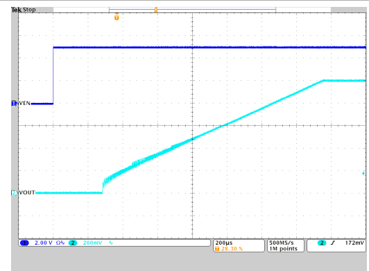
Figure 9-53. Start-Up Timing
