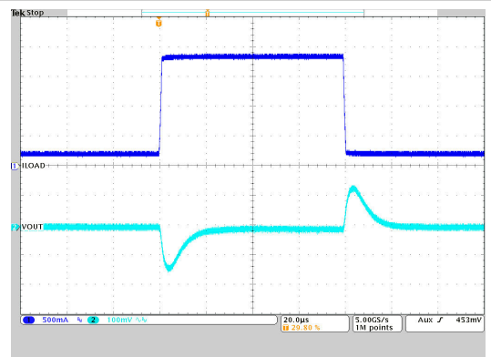
Figure 9-23. Load Transient Response
