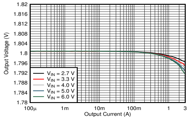
Figure 9-11. Output Voltage Versus Output Current
