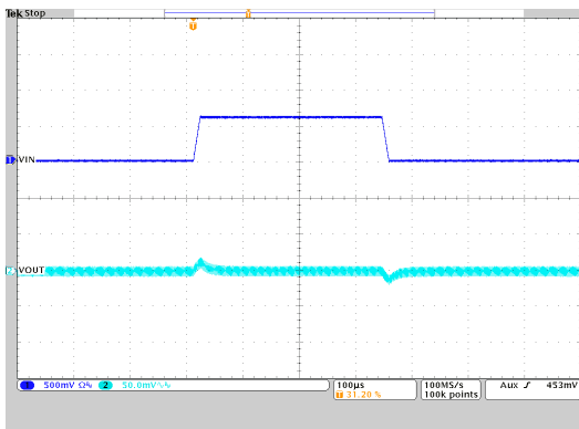
Figure 9-38. Line Transient Response
