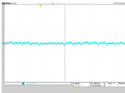
Figure 9-44. Output Voltage Ripple
