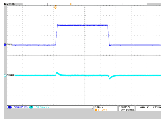
Figure 9-35. Line Transient Response
