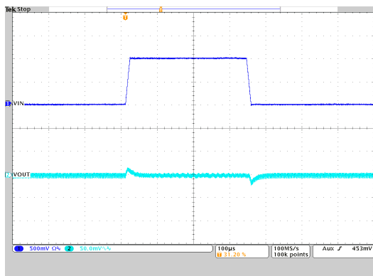
Figure 9-34. Line Transient Response
