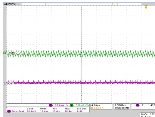
Figure 8-46. Output Voltage Ripple
