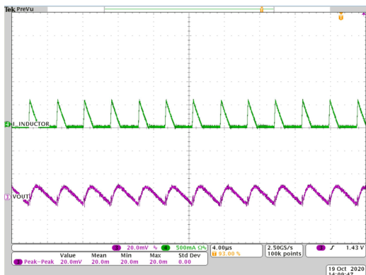
Figure 8-45. Output Voltage Ripple
