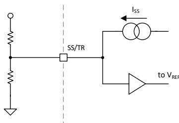
Figure 8-5. Tracking Operation Simplified Schematic
