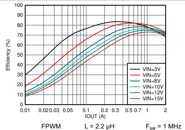
Figure 8-71. Efficiency vs Output Current V_{OUT} = 0.4\text{ V}
