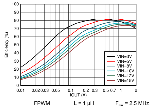
Figure 8-73. Efficiency vs Output Current V_{OUT} = 0.4\text{ V}
