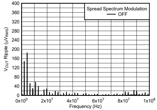
12V to 3.3V, 2A 1 \mu H, 2.2MHz First L-C only BW = 10kHz
