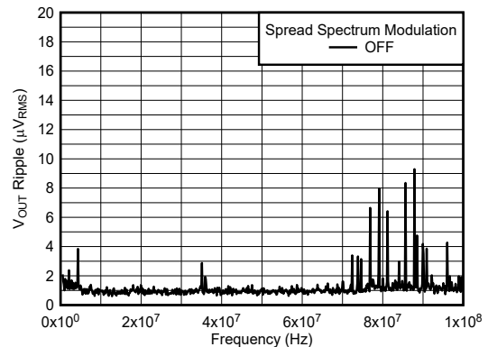
12V to 3.3V, 2A 1 \mu H, 2.2MHz First and second L-C BW = 10kHz
