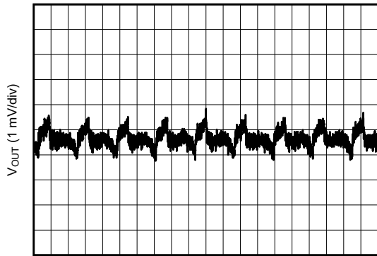
12V to 3.3V, 2A 1 \mu H, 2.2MHz First L-C only
