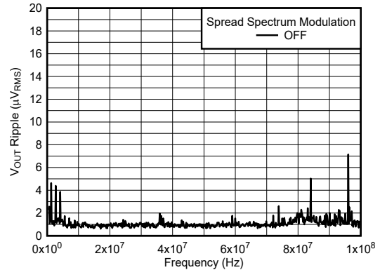
12V to 1.8V, 2A 1 \mu H, 1.4MHz First and second L-C BW = 10kHz
