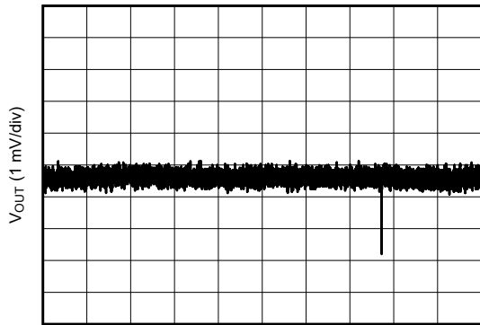
12V to 1.8V, 2A 1 \mu H, 1.4MHz First and second L-C
