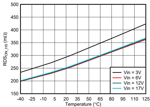
Figure 7-11. High-Side R_{DS(on)} vs Temperature
