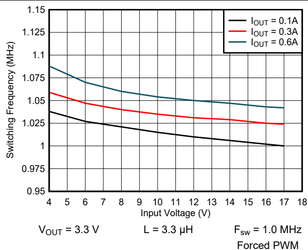
Figure 9-23. Switching Frequency vs Input Voltage
