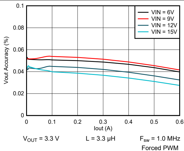
Figure 9-25. Output Voltage vs Output Current
