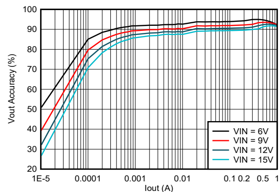
Efficiency vs Output Current V_{OUT} = 3.3 V at 1.0-MHz Auto PFM/PWM
