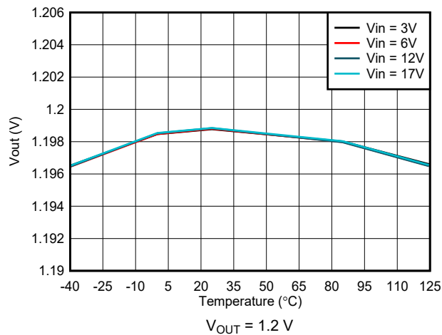
Figure 7-7. Output Voltage Accuracy – VSET Selected
