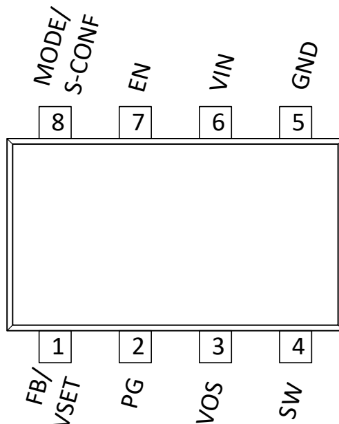
Figure 6-1. TPS629206 8-Pin DRL SOT-5X3 Pinout
