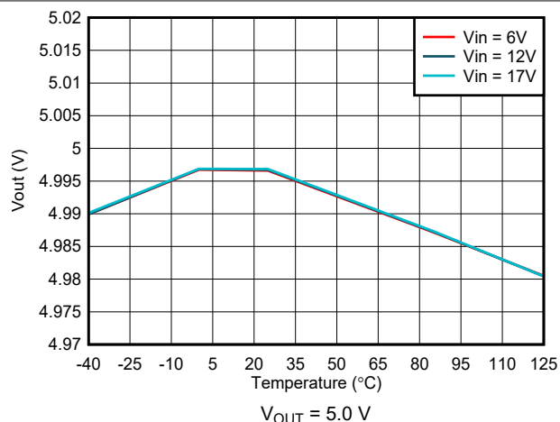
Figure 7-4. Output Voltage Accuracy – VSET Selected
