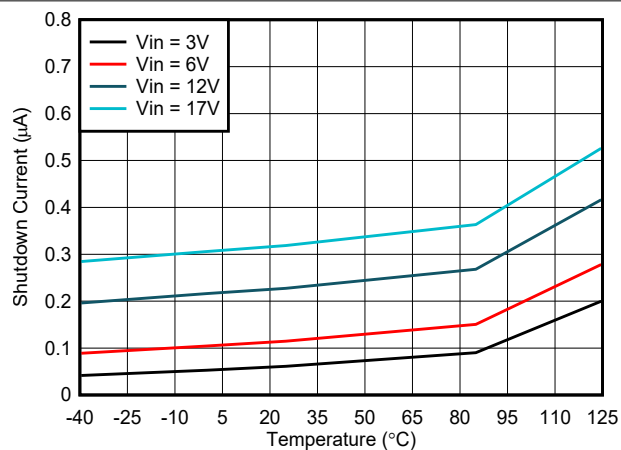
Figure 7-2. Typical Shutdown Current vs Temperature
