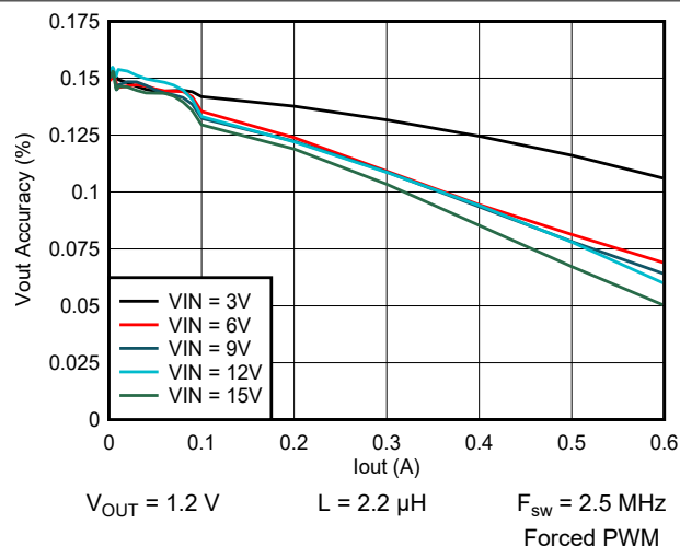
Figure 9-43. Output Voltage vs Output Current
