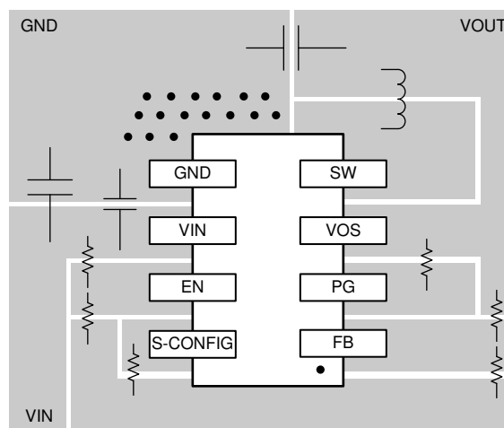
Figure 11-1. TPS629206 Layout
