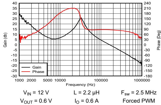
Figure 9-80. Bode Plot
