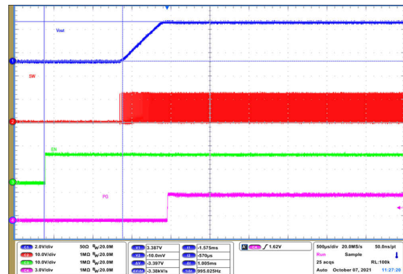
Figure 9-63. Start-Up Timing
