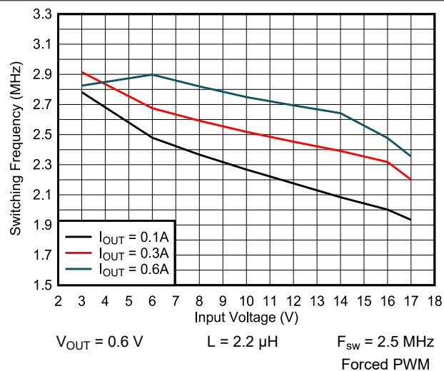
Figure 9-53. Switching Frequency vs Input Voltage
