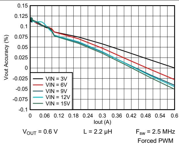
Figure 9-55. Output Voltage vs Output Current
