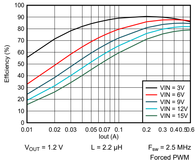
Figure 9-39. Efficiency vs Output Current
