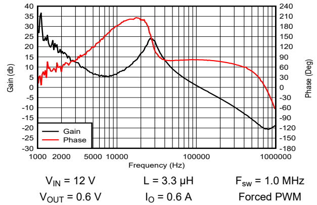
Figure 9-81. Bode Plot
