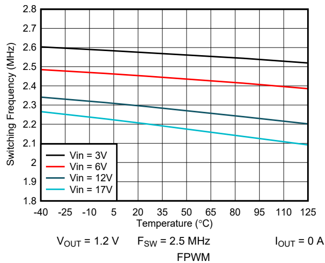
Figure 7-9. Switching Frequency vs Temperature
