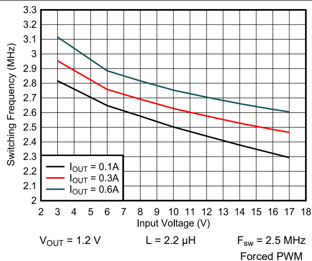
Figure 9-41. Switching Frequency vs Input Voltage
