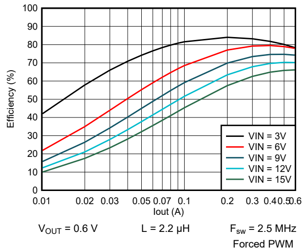
Figure 9-51. Efficiency vs Output Current
