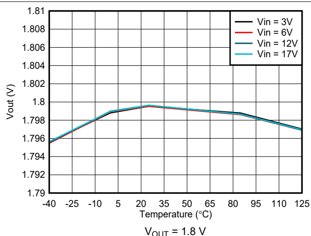
Figure 7-6. Output Voltage Accuracy – VSET Selected
