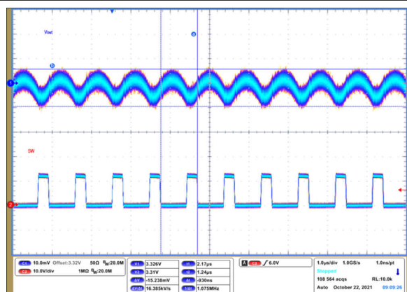
Figure 9-74. Output Voltage Ripple
