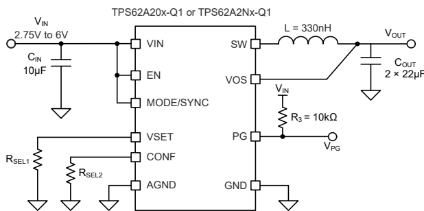
Simplified Schematic for TPS62A20x-Q1 and TPS62A2Nx-Q1
