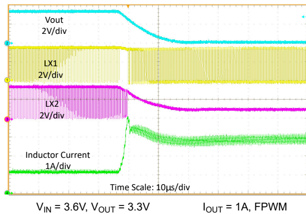
Figure 8-22. Output Short Protection (Entry)
