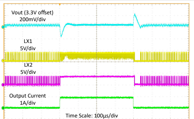
V_{IN} = 3.6V , V_{OUT} = 3.3V I_{OUT} = 100mA to 1A with 20\mu s slow rate
