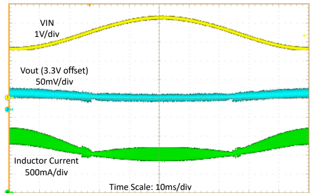
Figure 8-21. Line Sweep at 1A Load Current
