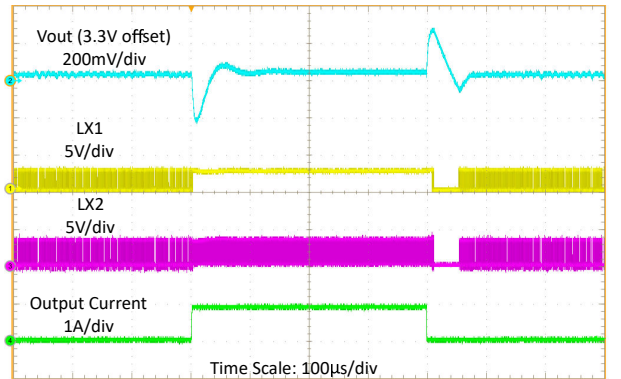
V_{IN} = 2.7V , V_{OUT} = 3.3V I_{OUT} = 100mA to 1A with 20\mu s slow rate
