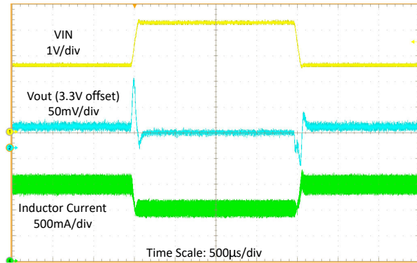
Figure 8-20. Line Transient at 1A Load Current
