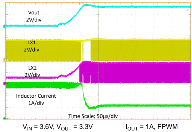
Figure 8-23. Output Short Protection (Recover)
