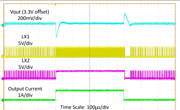
V_{IN} = 4.3V , V_{OUT} = 3.3V I_{OUT} = 100mA to 1A with 20\mu s slow rate
