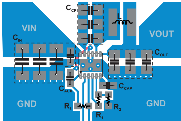
Figure 45. Recommended Layout
