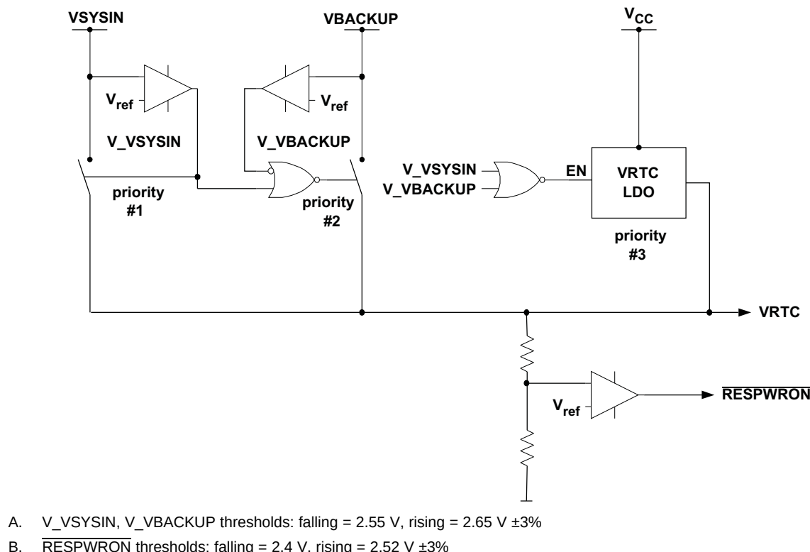
Figure 29. RTC and \overline{RESPWRON}
