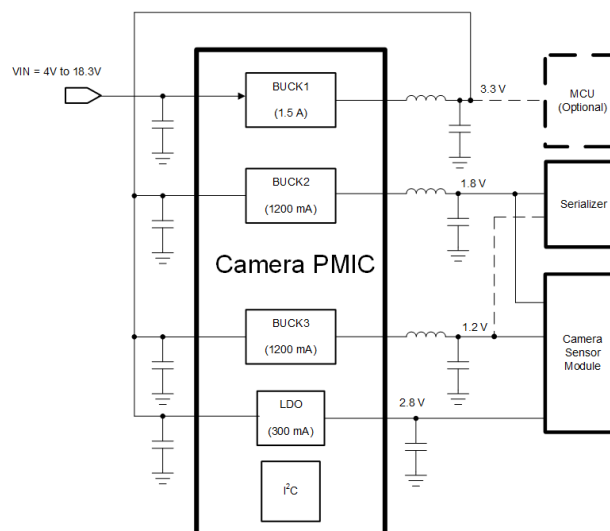
TPS650331-Q1 Application Circuit
