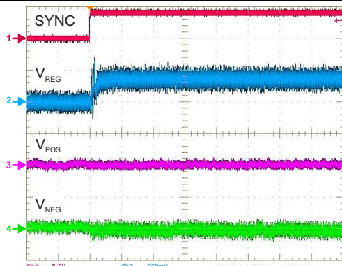
Figure 90. SYNC = HIGH (zoom)
