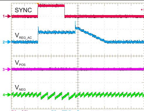
Figure 88. SYNC Signal — I_{OUT} = 10\text{ mA}
