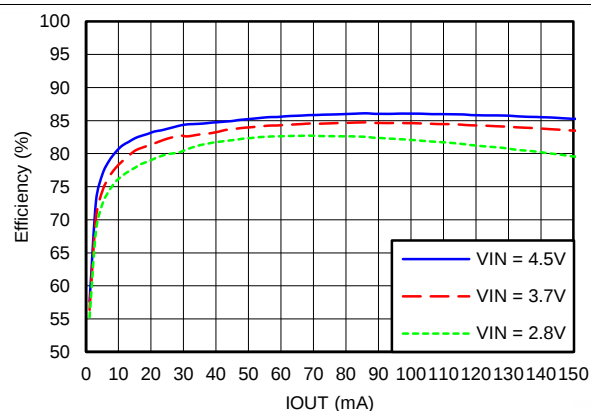
Figure 84. Combined Efficiency — \pm 5.4\text{ V} — SYNC = HIGH L = 2.2\text{ }\mu\text{H}
