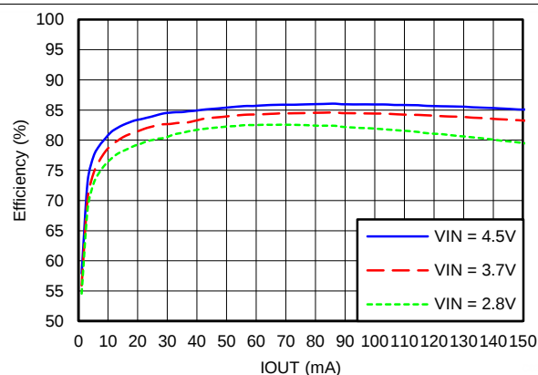
Figure 83. Combined Efficiency — \pm 5.0\text{ V} — SYNC = HIGH L = 2.2\text{ }\mu\text{H}
