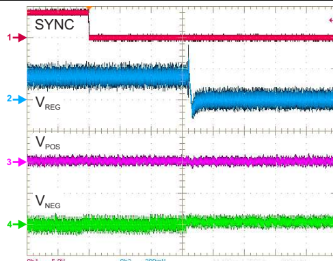
Figure 91. SYNC = LOW (zoom) with Delay
