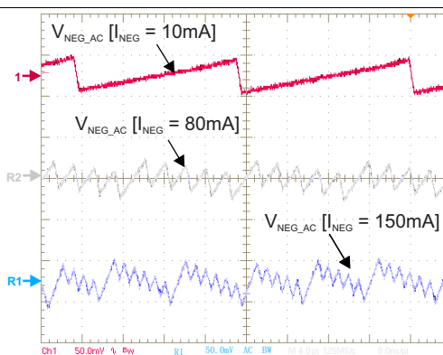
Figure 86. V_{\text{NEG}} Output Voltage Ripple — SYNC = HIGH — L = 2.2\text{ }\mu\text{H} — C_{\text{OUT}} = 10\text{ }\mu\text{F}
