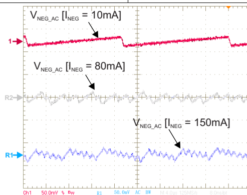
Figure 87. V_{\text{NEG}} Output Voltage Ripple — SYNC = HIGH — L = 2.2\text{ }\mu\text{H} — C_{\text{OUT}} = 2 \times 10\text{ }\mu\text{F}
