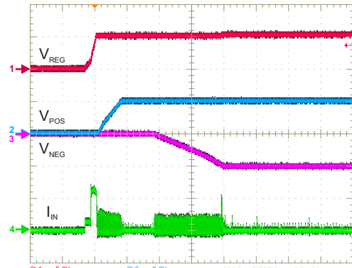
Figure 107. Inrush Current — Sequential SYNC = HIGH
