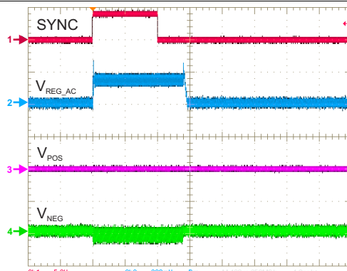
Figure 89. SYNC Signal — I_{OUT} = 150\text{ mA}
