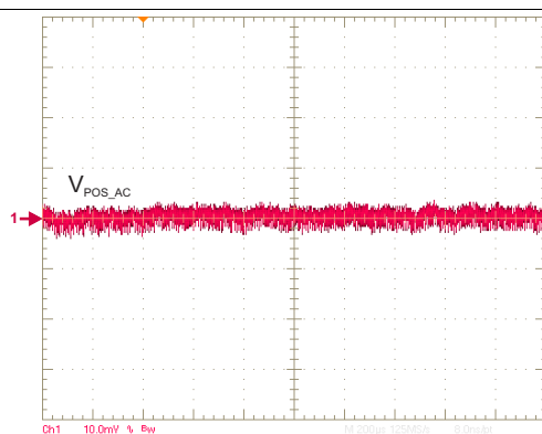
Figure 85. V_{\text{POS}} Output Voltage Ripple — SYNC = HIGH
