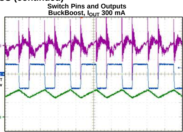
400 ns/div Figure 6.
