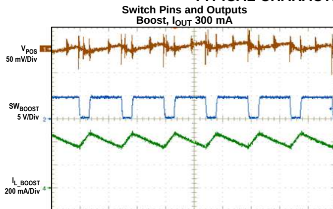
400 ns/div Figure 5.
