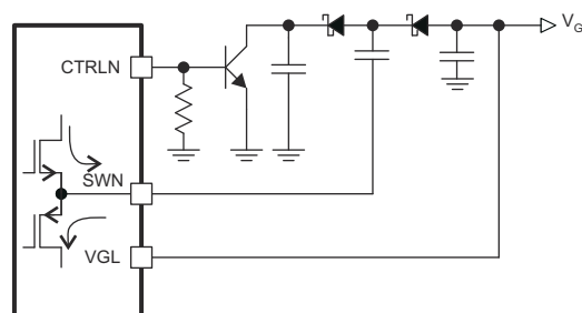
Figure 8-2. Negative Charge Pump Application Circuit
