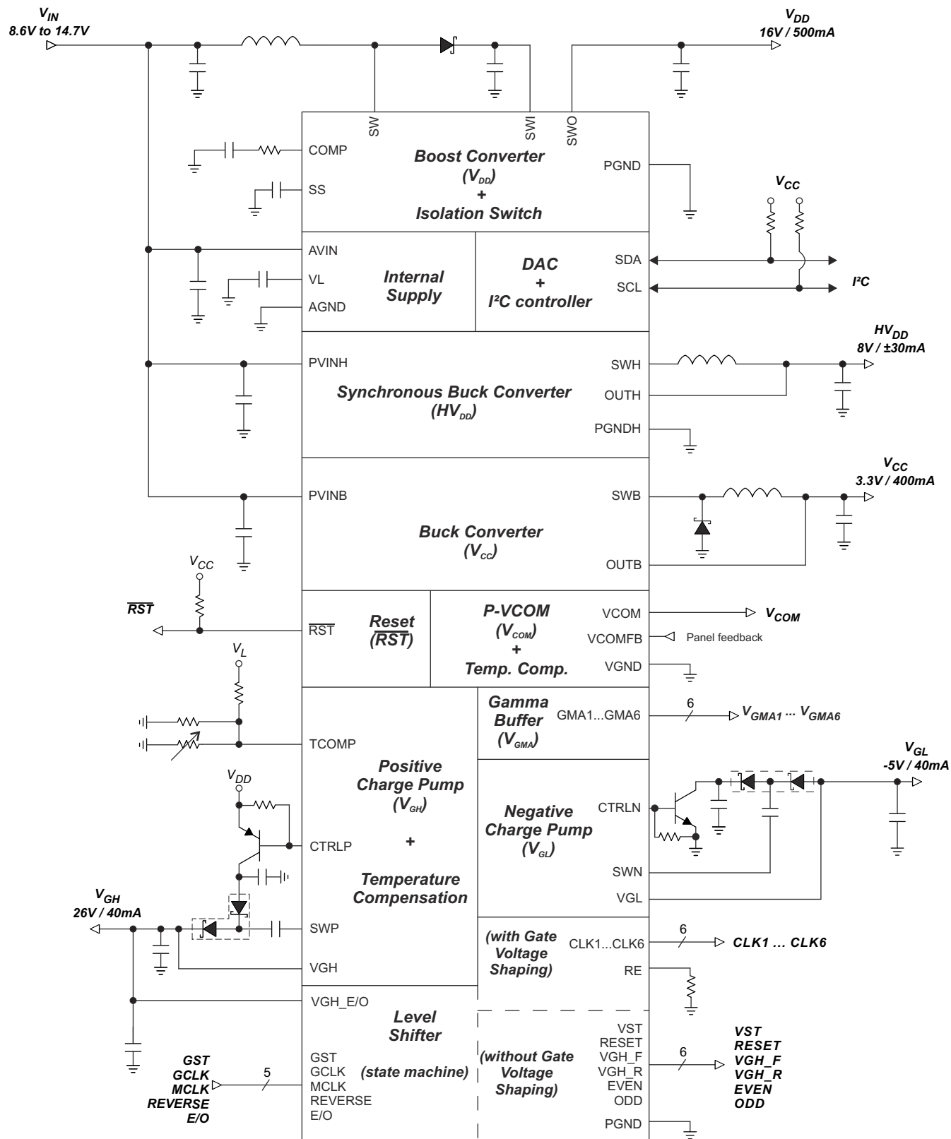
Figure 6-2. Simple Application Schematic
