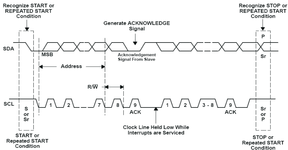
Figure 9-5. Bus Protocol
