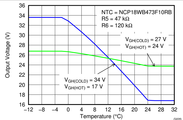
Figure 6-19. TEMPERATURE COMPENSATION VOLTAGE ADJUSTMENT
