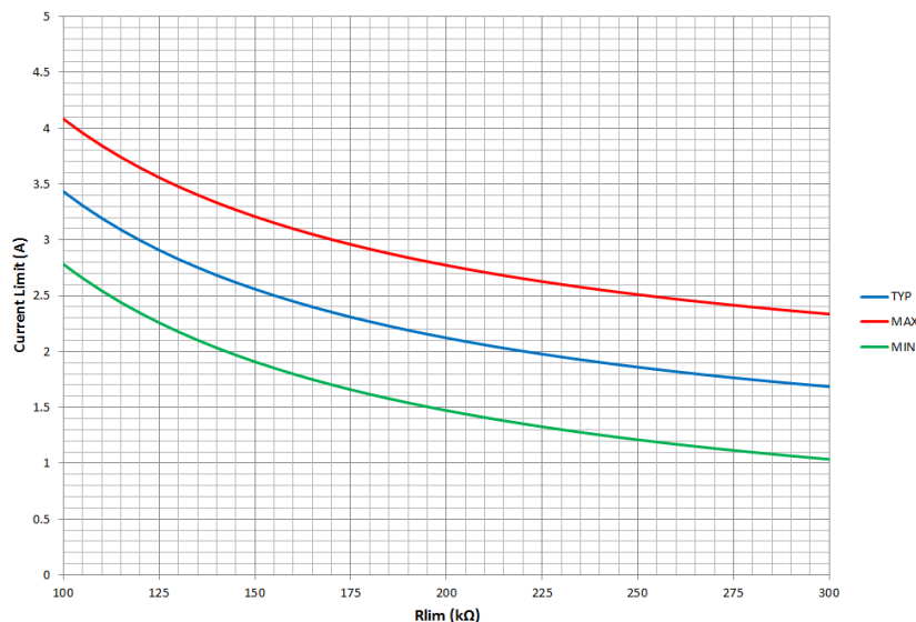
Figure 34. Buck 2
