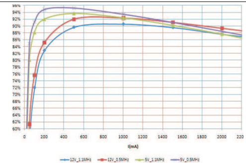
Figure 2. BUCK1 Efficiency
