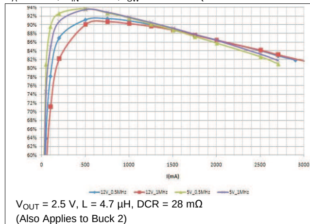
Figure 7. BUCK3 Efficiency
